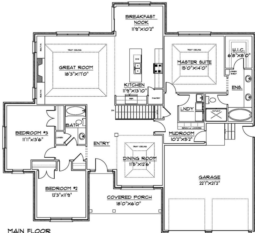
MAIN FLOOR 2170 sqft
