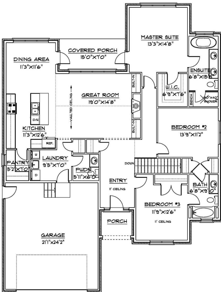
MAIN FLOOR 1956 SQ. FT.
